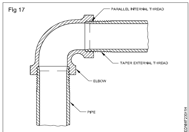
Pipe threads (Fig 17)
