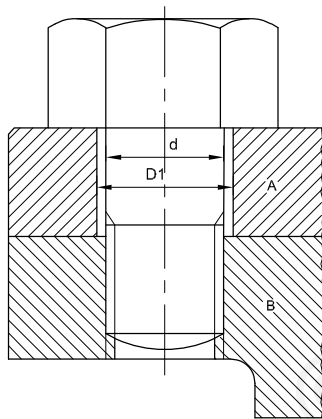
TAP - BOLT OR CAP - SCREW
