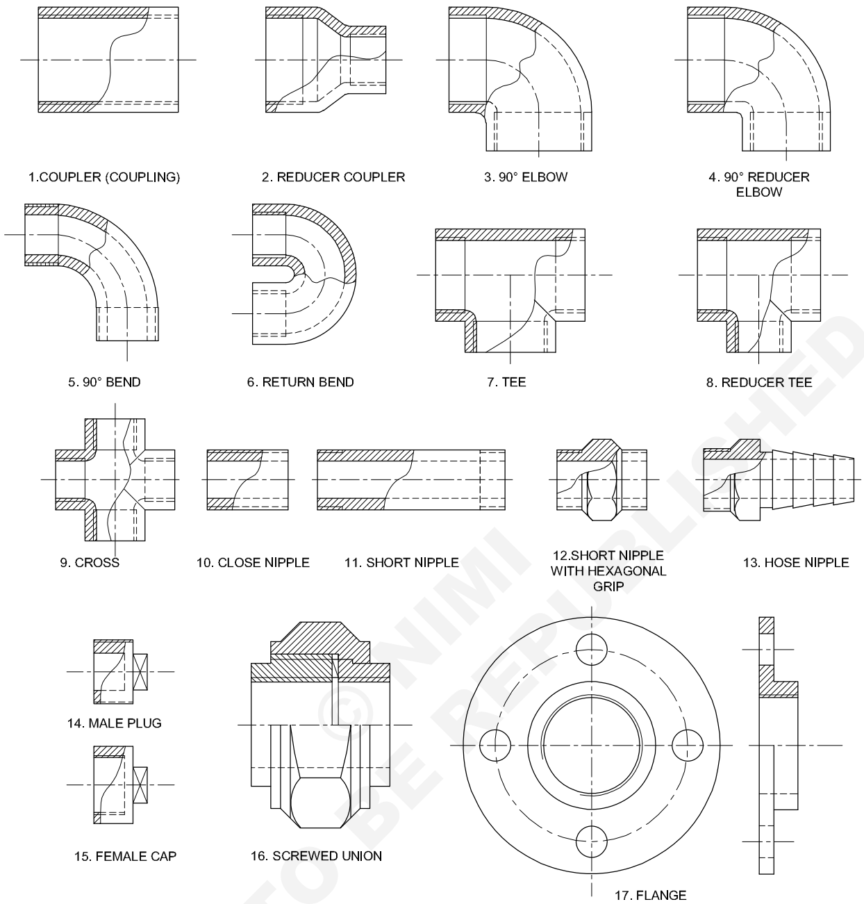
PIPE FITTINGS
